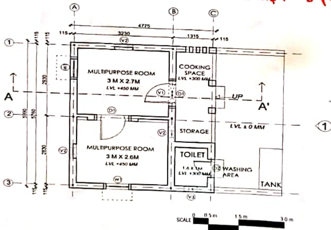
TYPICAL PLAN
